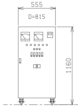
Xenon Ballast
